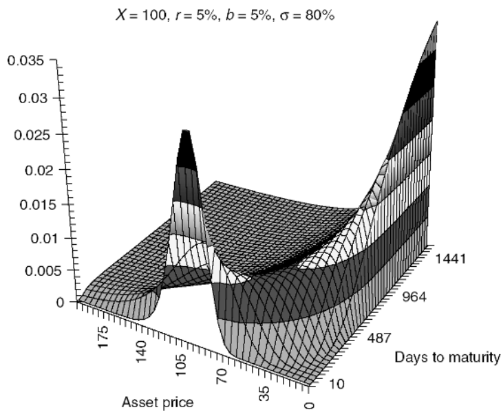
Figure 4: Saddle gamma
