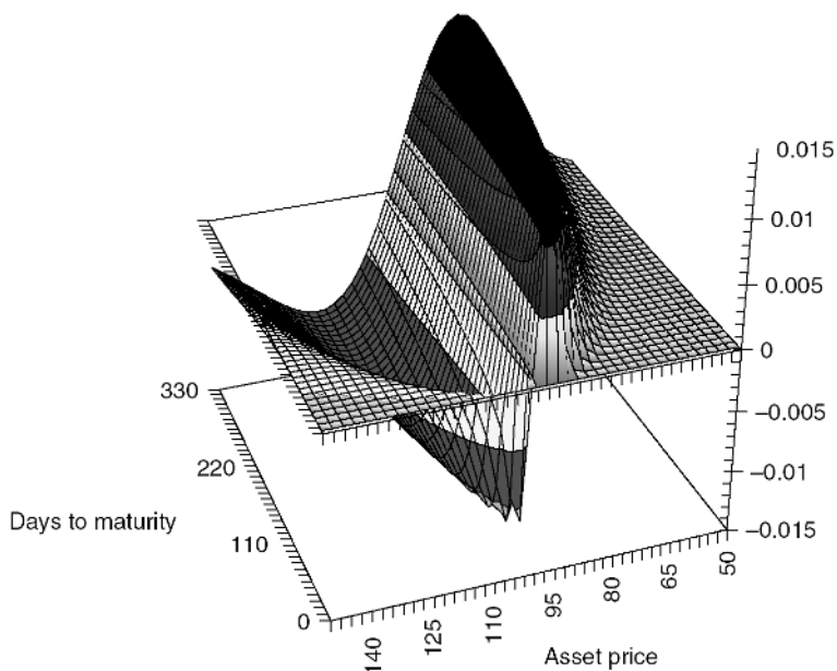
Figure 2: DdeltaDvol
