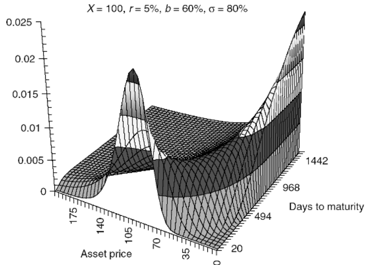
Figure 6: Saddle gammaP
