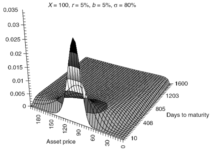
Figure 5: GammaP
