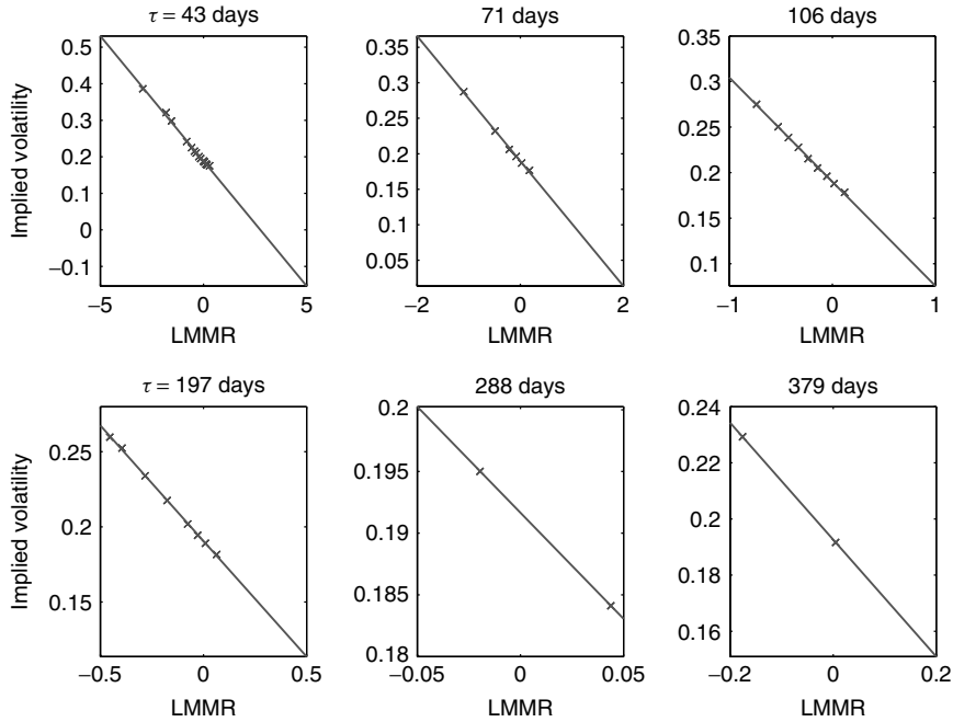
Figure 1: S&P500 implied volatility data on June 5, 2003 and fits to the affine LMMR approximation (4) for six different maturities
