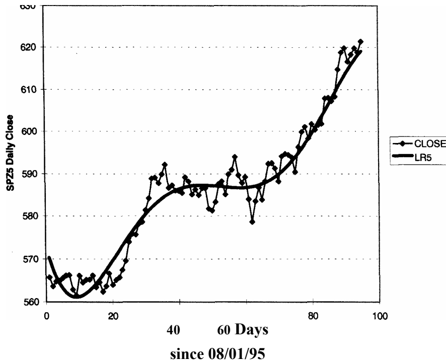
Figure 2.2 SScP-500 closing data with regression using terms raised to the fifth power.
