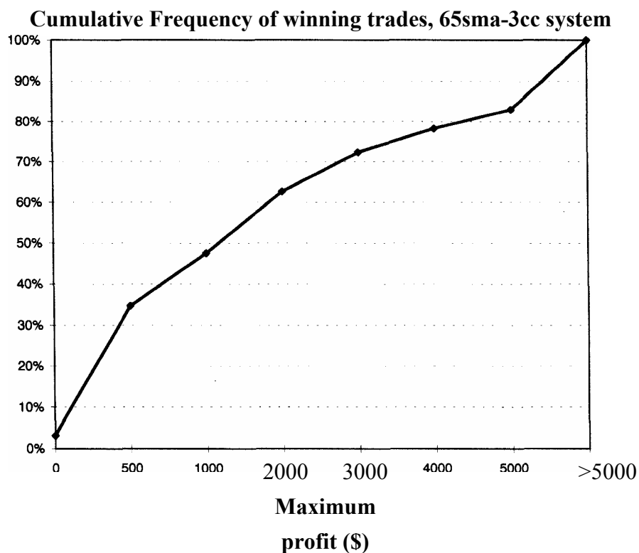
Figure 4.11 Cumulative frequency of maximum favorable excursion of 65sma-3cc system. Note that horizontal scale is not linear.
